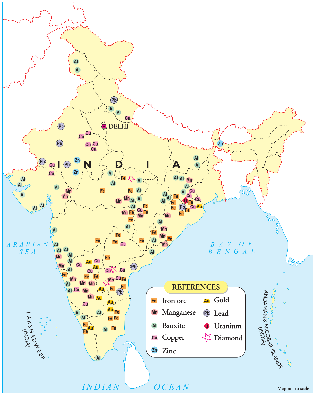
mineral resources in India
