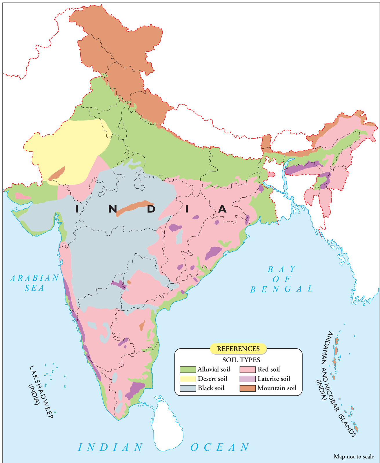
soil types of India
